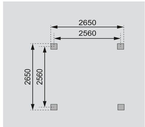
Fundamentplan Pfosten (in mm)
