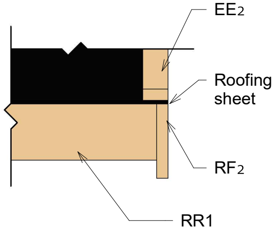
③ Roof Reinforcement
