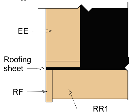
3 Roof Reinforcement
