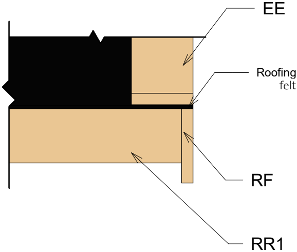
3 Roof Reinforcement
